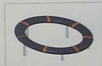
SUPERNOVA
