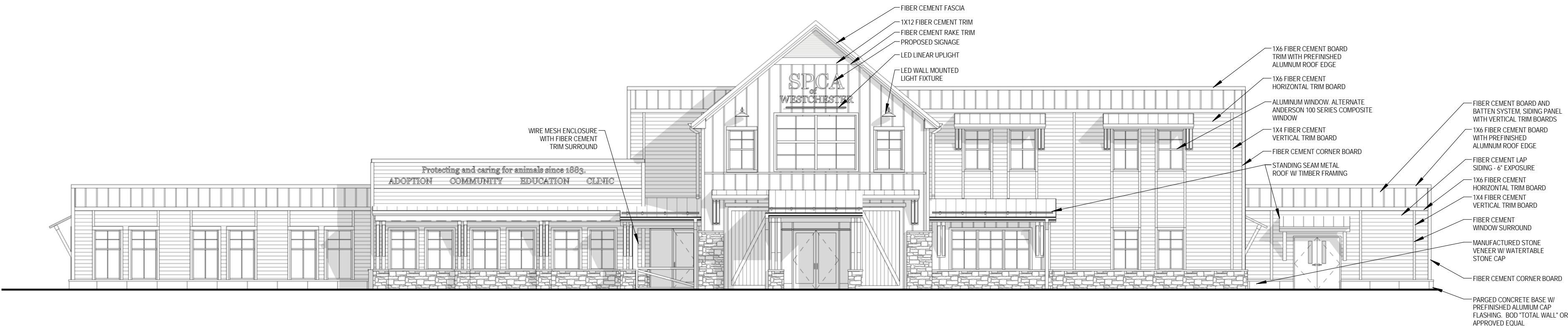
1 FRONT ELEVATION 3/32" = 1'-0"
