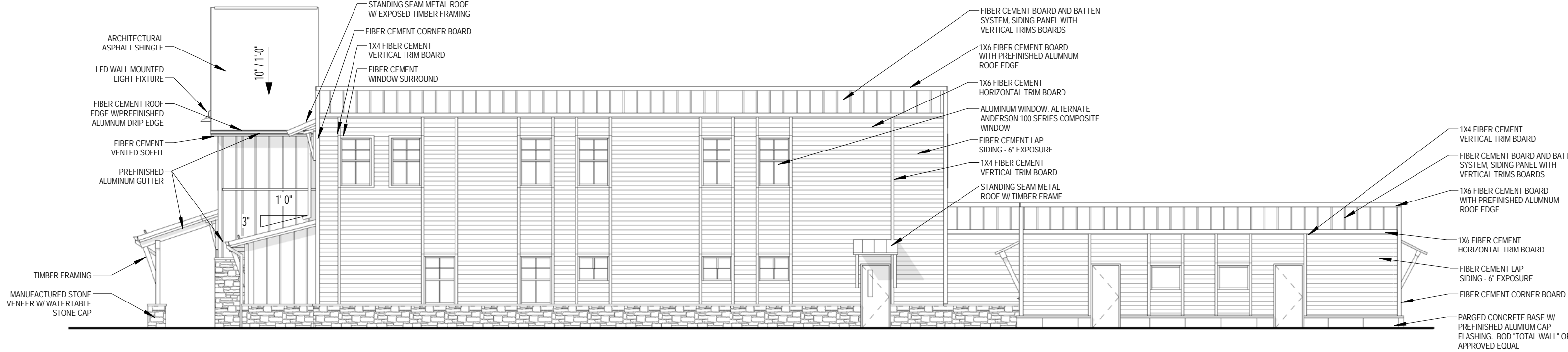
4 RIGHT ELEVATION 3/32" = 1'-0"
